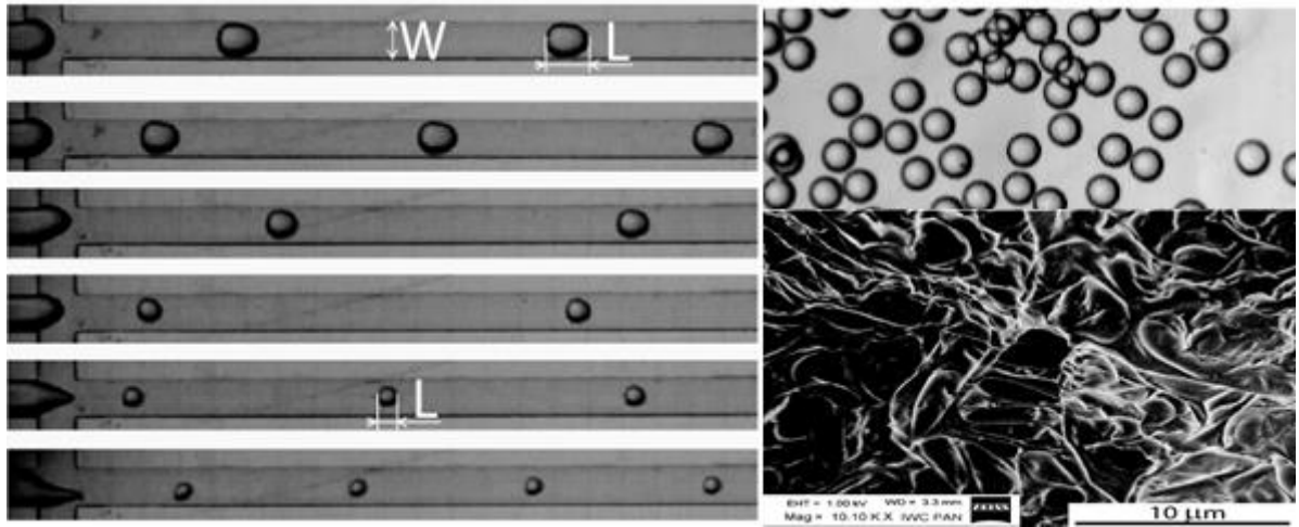
Fig. Micrographs of generation of aqueous pectin solution droplets in continuous phase (left). In turn, micrograph illustrating pectin microbeads and scanning electron micrograph of their surface are presented on the right.
